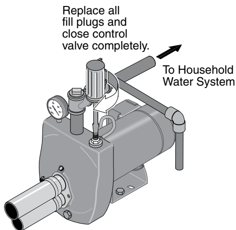
Figure 13: Prime Pump
