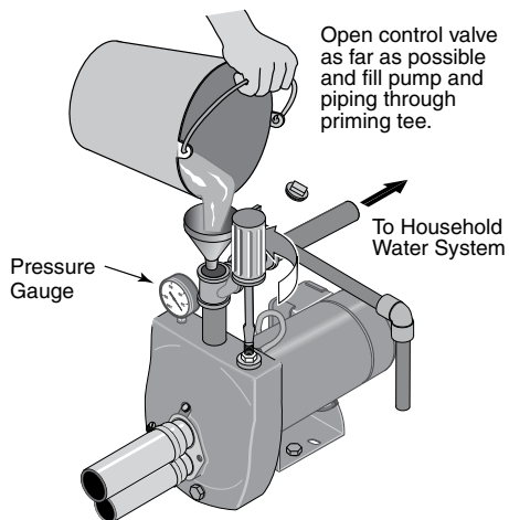
Figure 12: Fill Pump
